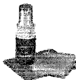
KK-LC3
